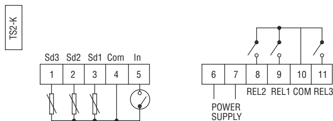
TSXT-XX3 3 relay outputs
